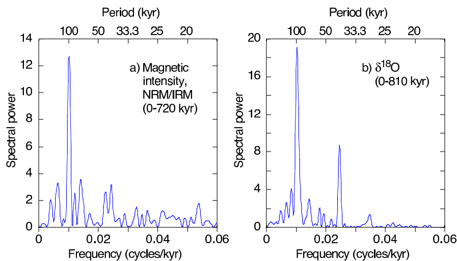
Fig. 4: Spectral powers of a) the geomagnetic paleointensity (mean NRM/IRM) of site 983 [23], and b) the \delta^{18}\text{O} in the benthic stack of Kerner et al. [50].
